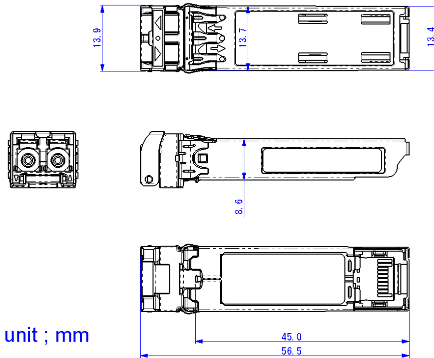
Figure 3. Package dimensions
