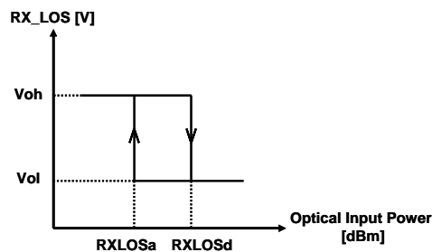
Figure.8. Optical Input Power vs. RX_LOS
